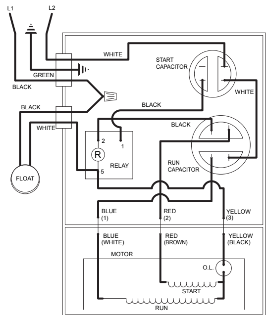
WIRING DIAGRAM FOR MODELS "WD820" All Revisions and "WH820" All Revisions 9/96 thru Current
