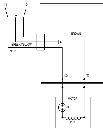
WIRING DIAGRAM FOR MODELS "N55", "N55-A", "N55-B", "N55-C" 9/82 (VN) thru Current
