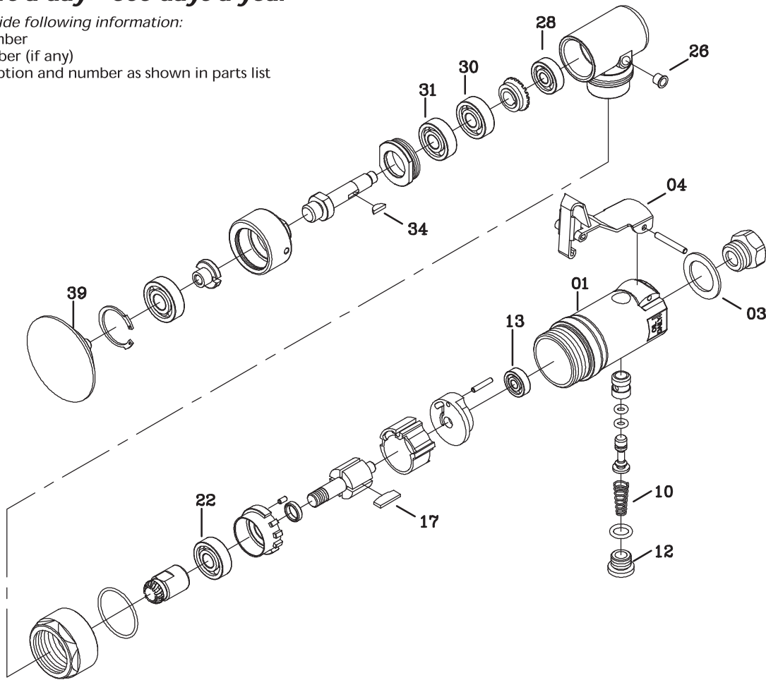
Figure 3 - Repair Parts Illustration for Mini Angle Orbital Sander
