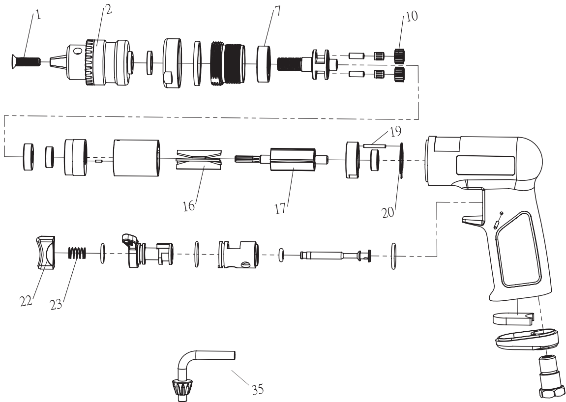
Figure 3 - Repair Parts Illustration for 1/4" Mini Air Reversible Drill
