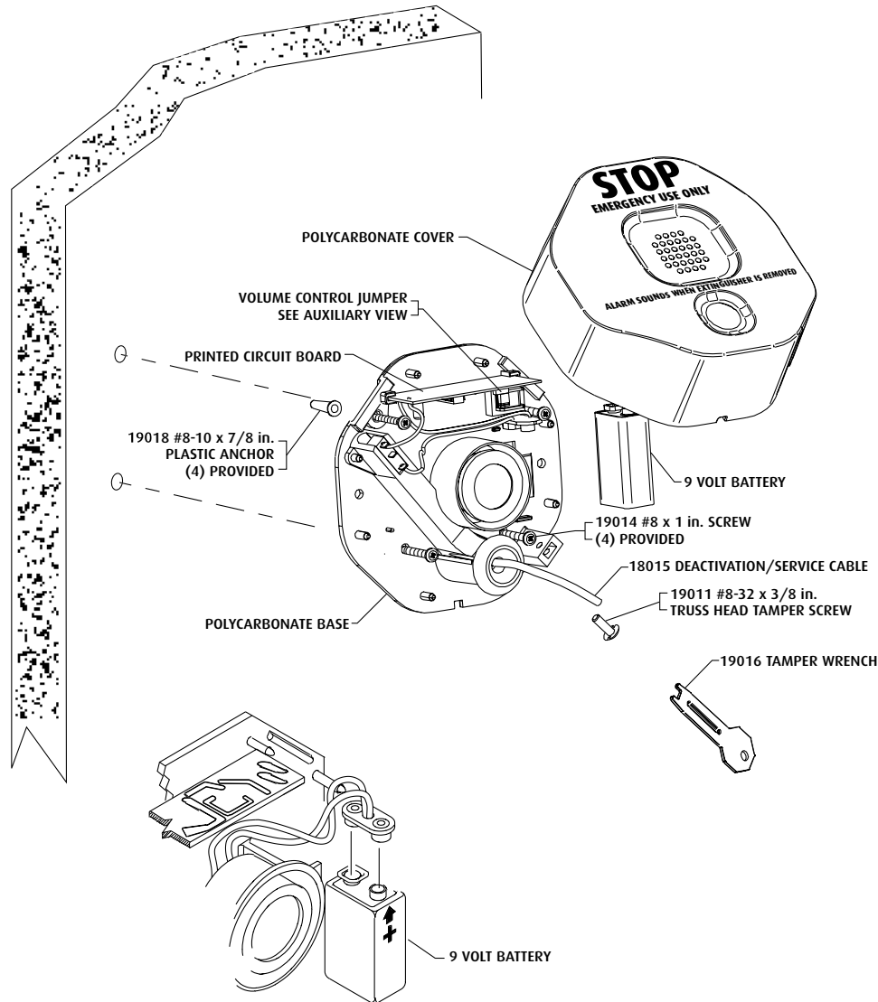
VIEW SHOWING BATTERY REPLACEMENT
