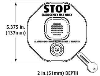
PRODUCT DIMENSIONS
