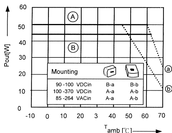
SDP3-15-100T
