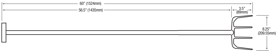
Model 2075
