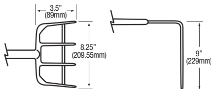
Model 2075R
