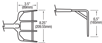
Model 2075SR
