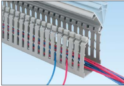
Type HN: Narrow Slot
