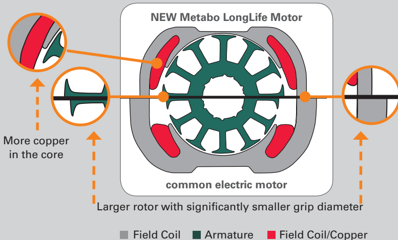
Cross-section electric motor
