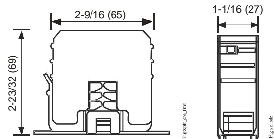
Figure 1: CTD Dimensions, in. (mm)
