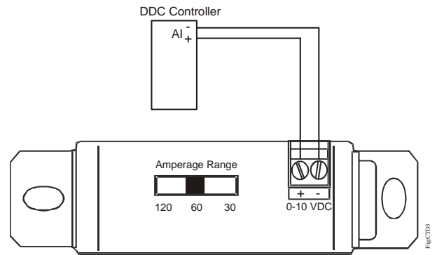
Figure 8: CTD-C3H00-1
