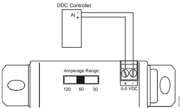
Figure 7: CTD-2G00-1
