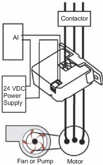
Figure 2: Model CTD-C1G00-1
