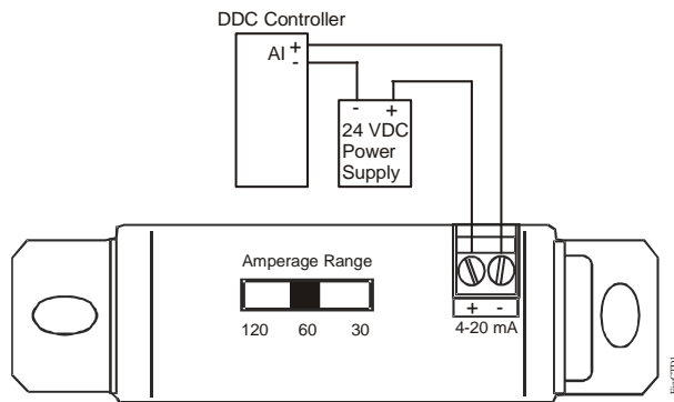
Figure 6: CTD-C1G00-1
