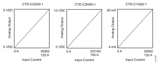
Figure 9: Transducer Linear Outputs
