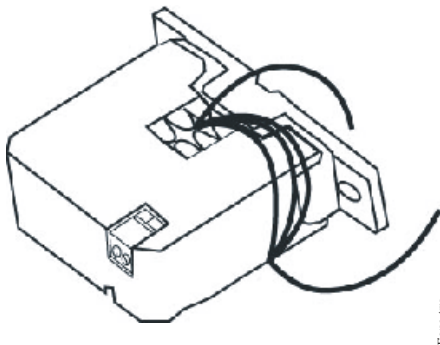
Figure 3: CSD Device Shown with Four Turns
