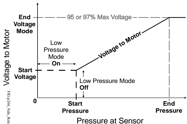
Figure 5: Relationship between P266 Series Control Variables
