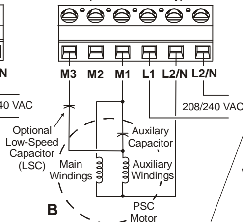
Two Triac with LSC Wiring for P266E Type Controls (208/240 VAC Only)
