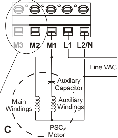
One Triac Wiring for P266A, P266B, and P266C Type Controls (208/240 VAC, 380/460 VAC, and 460/575 VAC)
