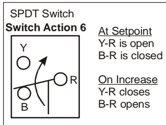
A19D Series Control Switch Action
