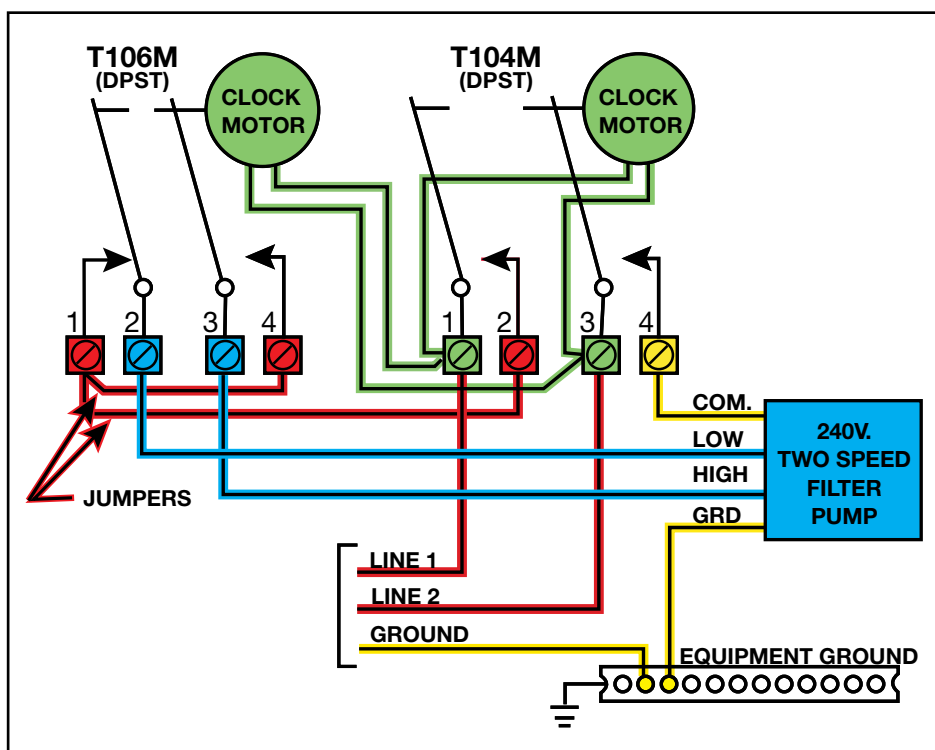
Rear View T104M – T106M
