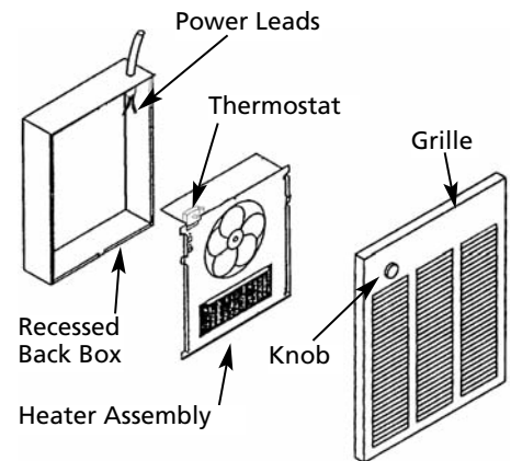
Figure 5 – Heater Assembly and Grille
