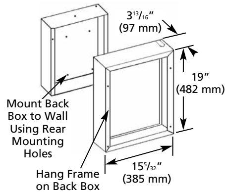
Figure 4 – Surface-Mounting Installation
