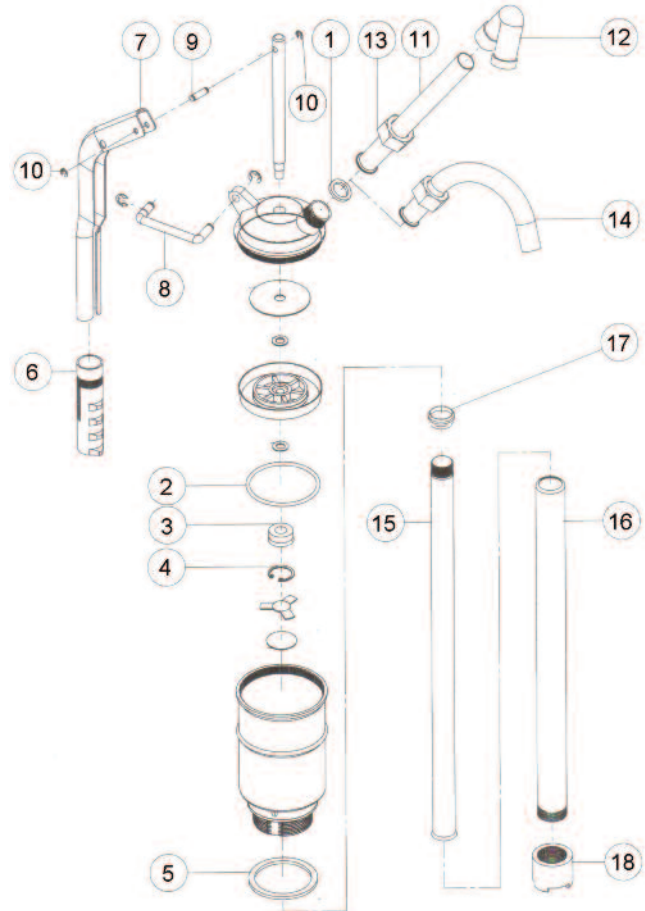
Figure 2 – Repair Parts Illustration for High Viscosity Lever Action Pump
