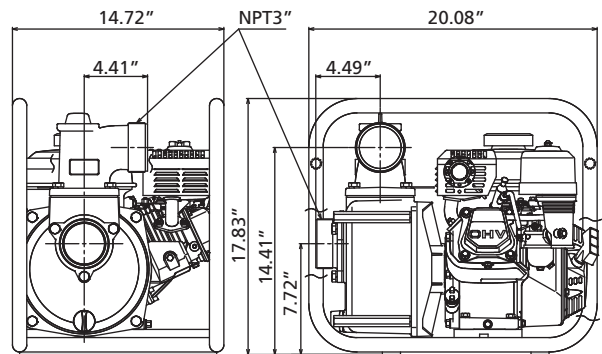
Dimensions for Model 11G235
