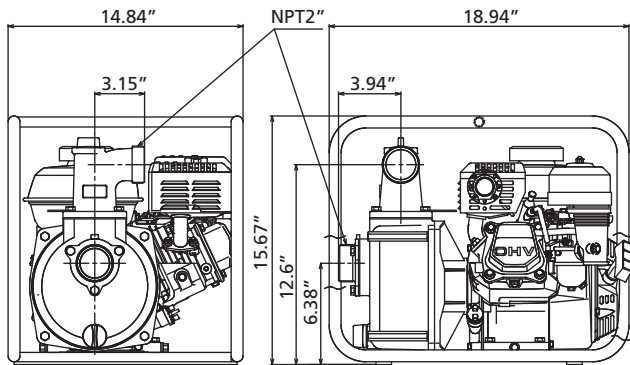
Dimensions for Model 11G234
