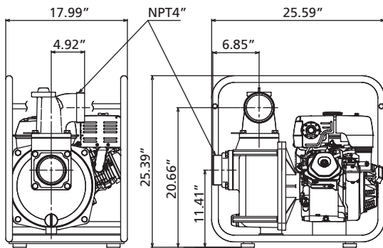
Dimensions for Model 11G236
