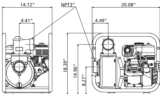
Dimensions for Model 11G229
