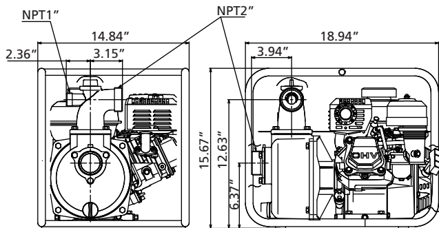
Dimensions for Model 11G227
