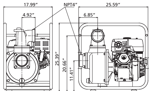
Dimensions for Model 11G230
