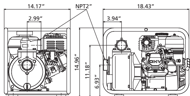
Dimensions for Model 11G228
