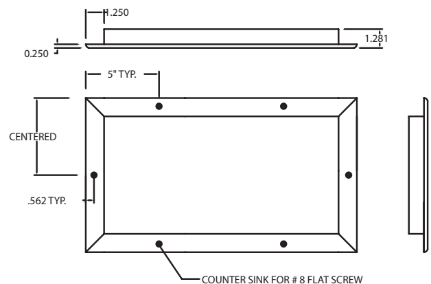
SLIP FIT COLLAR Figure 2
