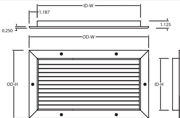
DOOR LOUVER Figure 1
