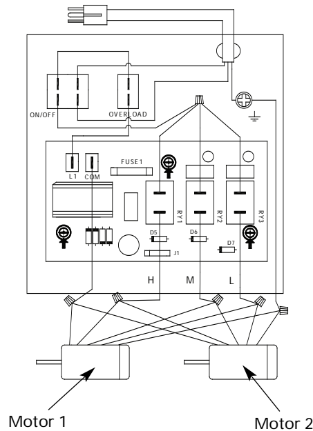
Figure 4 - Electrical Circuit Diagram
