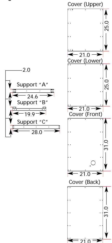
Figure 3 - Dimensions of Covers and Supports
