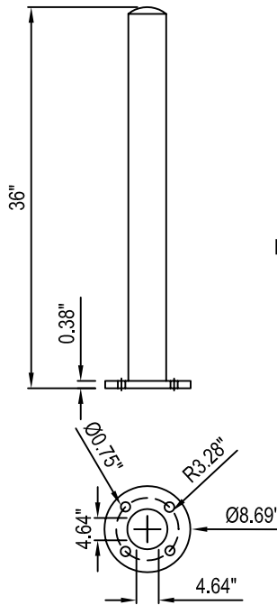
PLAN VIEW - BASE PLATE
