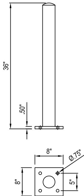
PLAN VIEW - BASE PLATE
