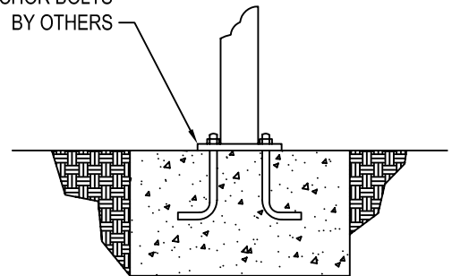
END VIEW - FOUNDATION
