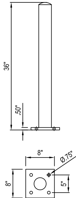
PLAN VIEW - BASE PLATE
