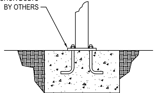
END VIEW - FOUNDATION
