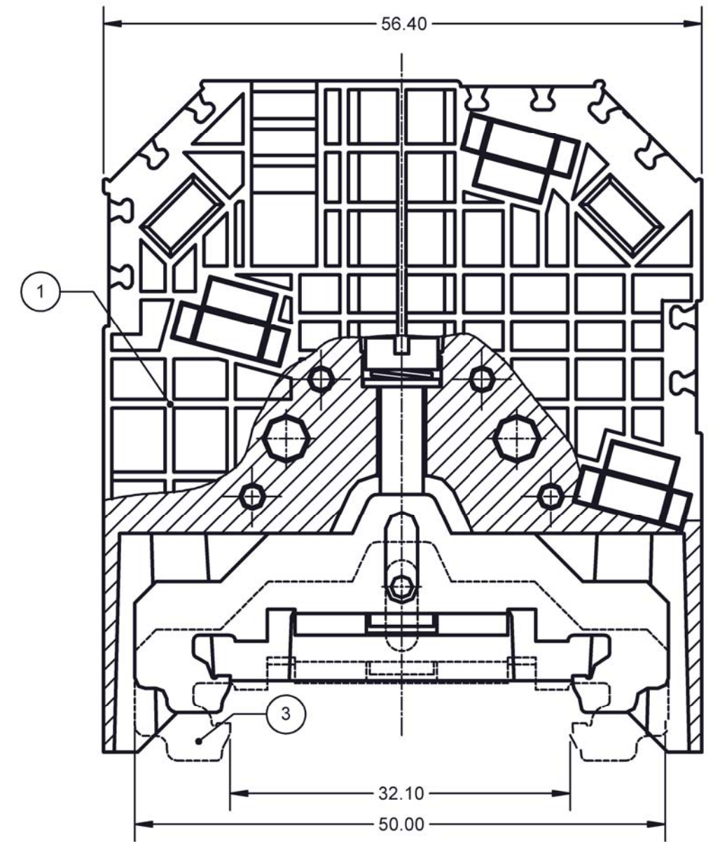
SECTION B-B
