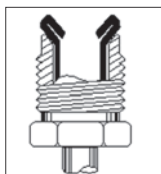
Flare tubing SAE (double) 7/16" - 24 thread
