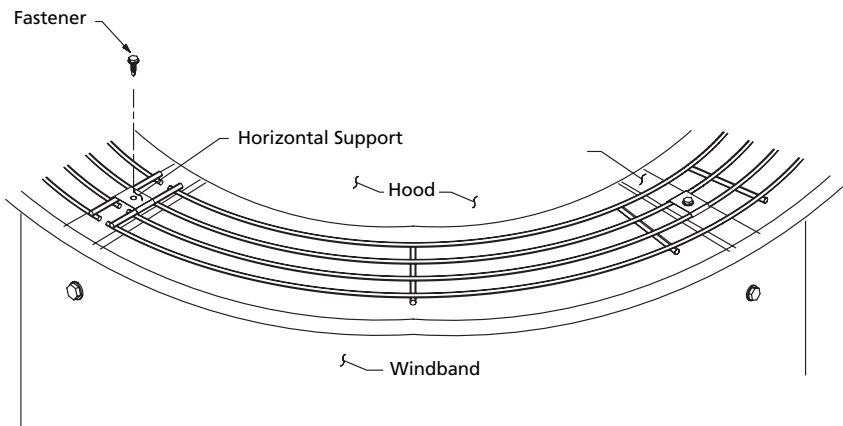
Figure 1 - Attaching Birdscreen
