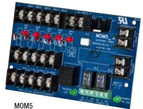
MOM5
