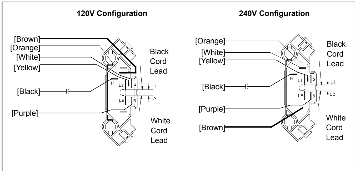
Figure 4 - 120V and 240V Configuration
