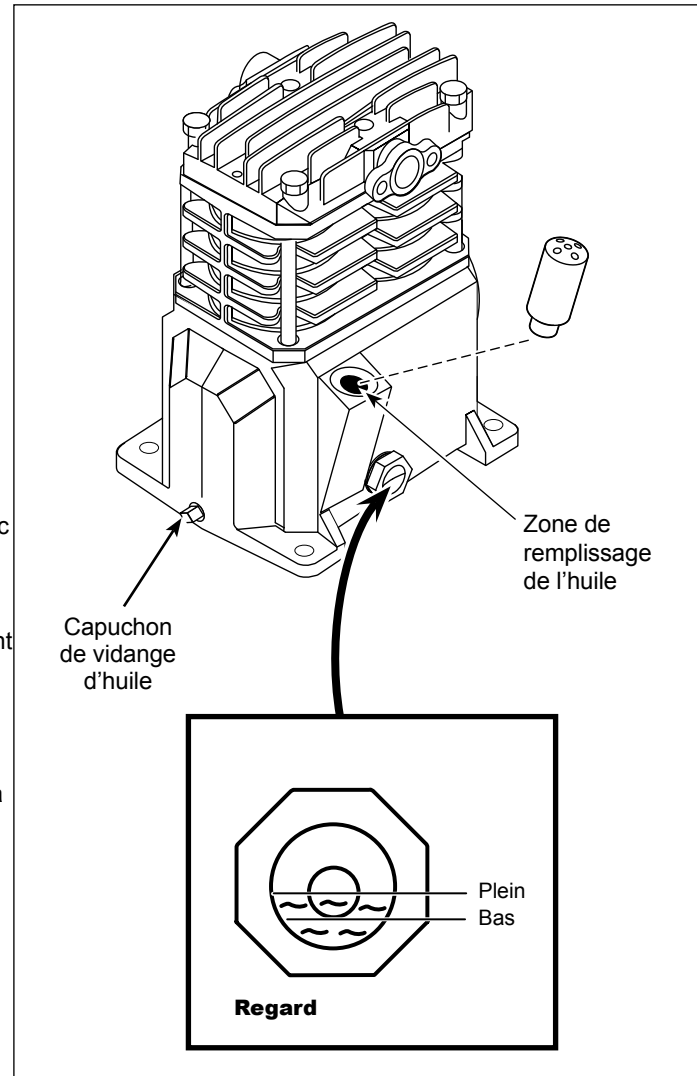
Figure 5 - Graissage
