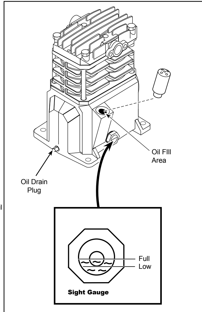
Figure 5 - Lubrication
