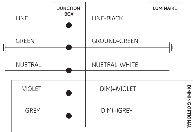
SUPPLY WIRING
