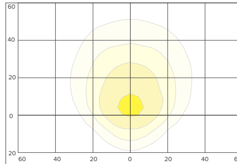
20' Mounting Height 5.0 FC, 2.0 FC, 1.0 FC, 0.5 FC
