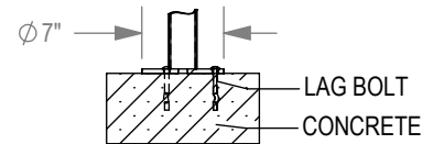
□ SURFACE FLANGE MOUNT (SF)
