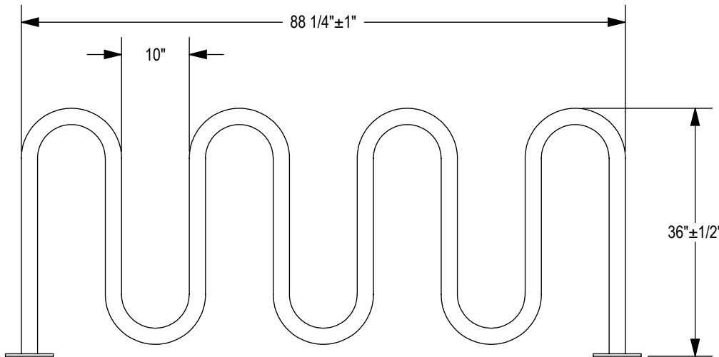
ELEVATION VIEW 7 LOOP - 9 BIKE CAPACITY
