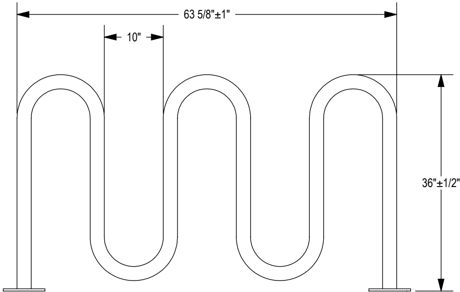
ELEVATION VIEW 5 LOOP - 7 BIKE CAPACITY
