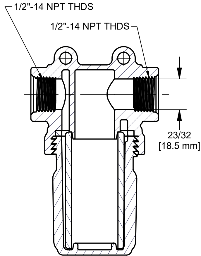
SECTION A-A SCALE 3 / 4
