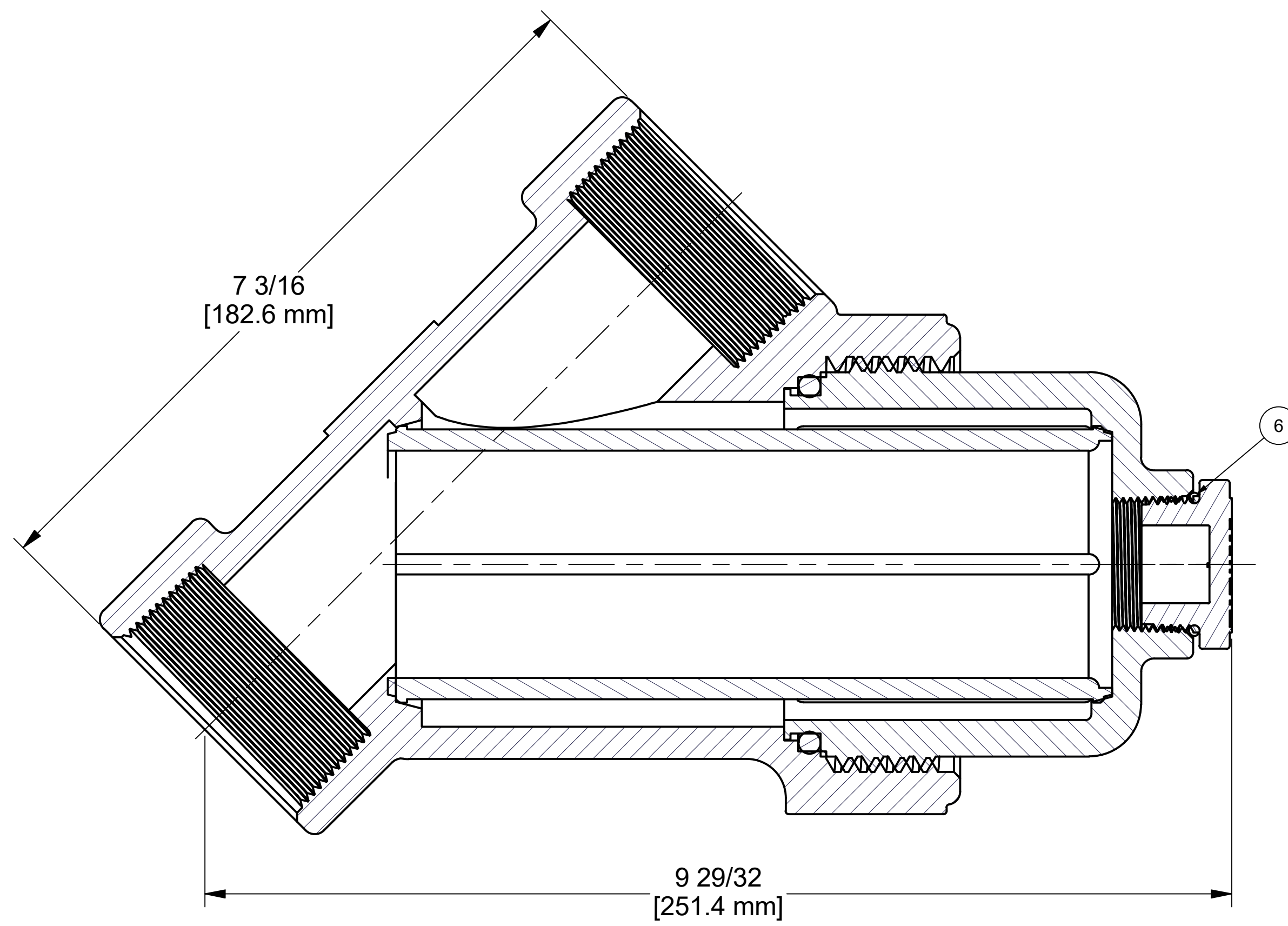
SECTION B-B SCALE 1 : 1
