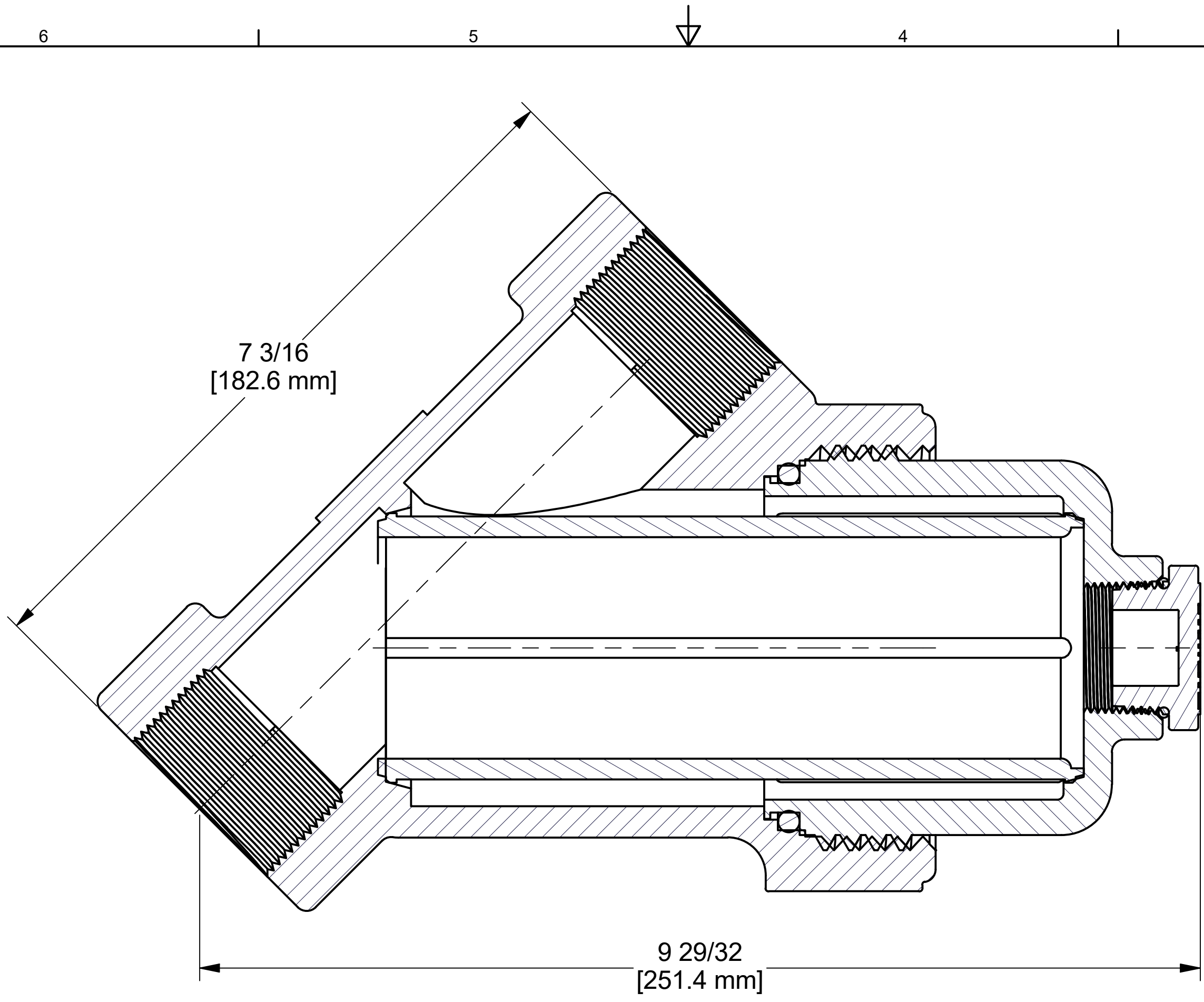
SECTION B-B SCALE 1 : 1
