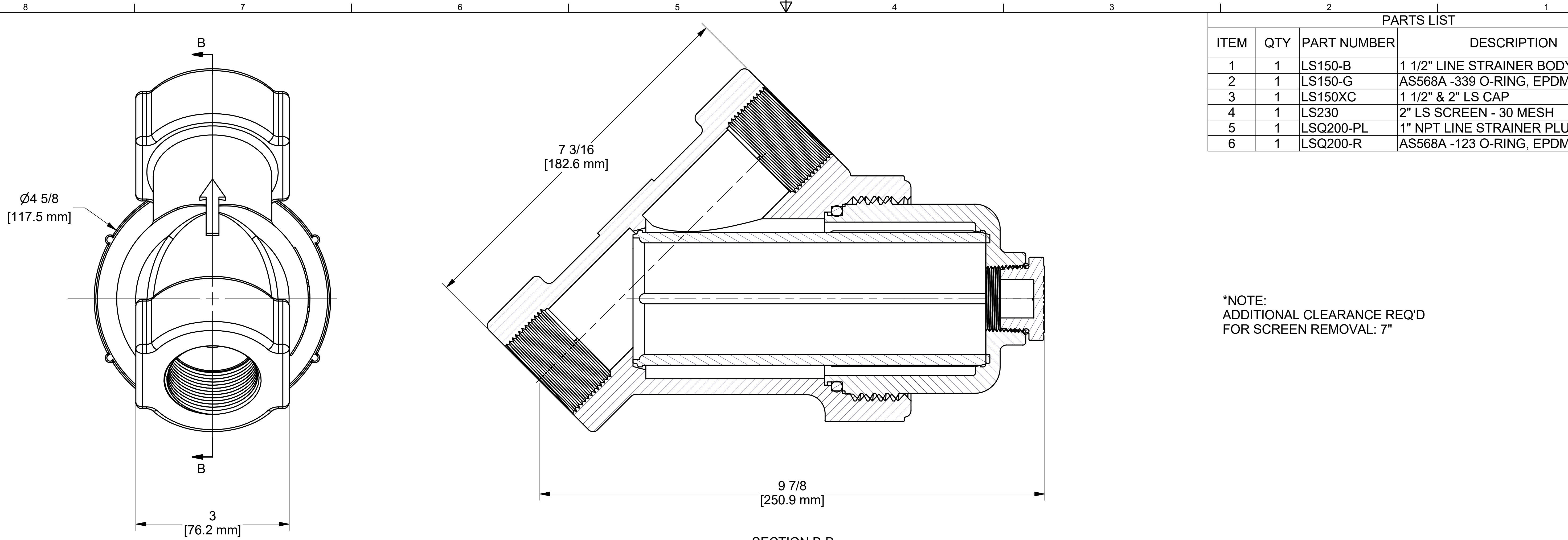
SECTION B-B SCALE 1 : 1
