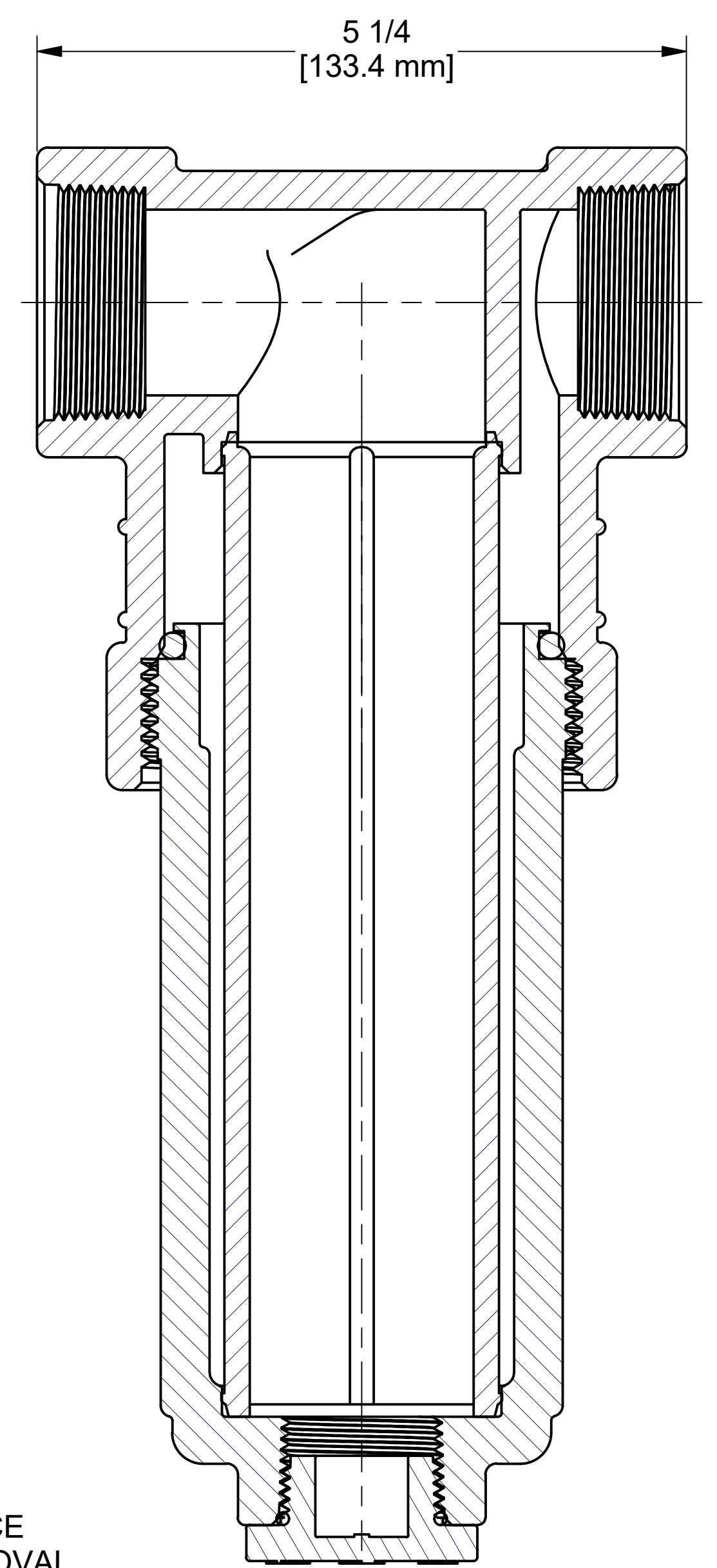
SECTION B-B SCALE 1 : 1
