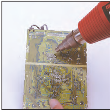
Desolder
