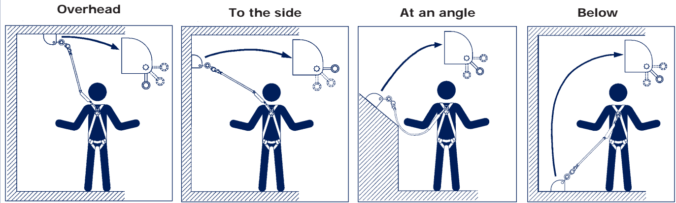
Figure 8 - Bracket Orientations
