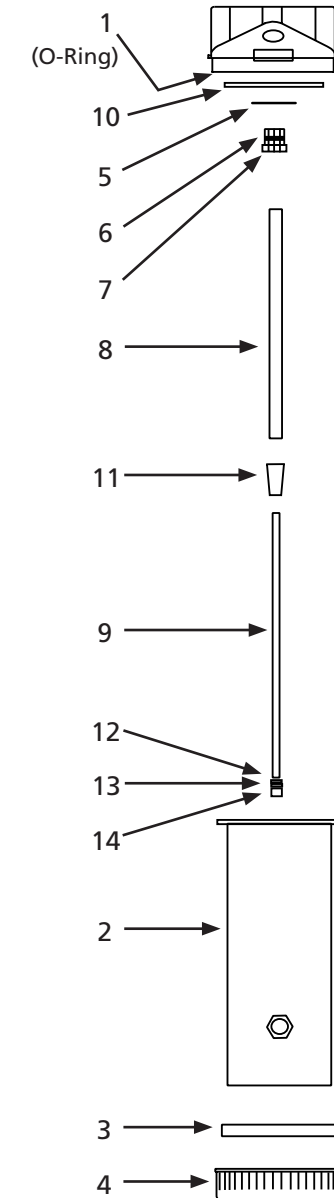
Figure 5 – Repair Parts Illustration for Desiccant Dryer
