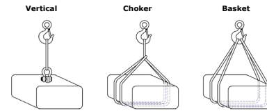
Figure 4-1. Common types of sling hitches
