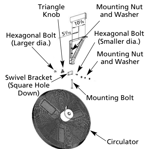
Figure 4 - Ceiling Mounted Assembly
