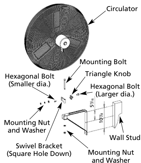
Figure 3 - Wall Mounted Assembly
