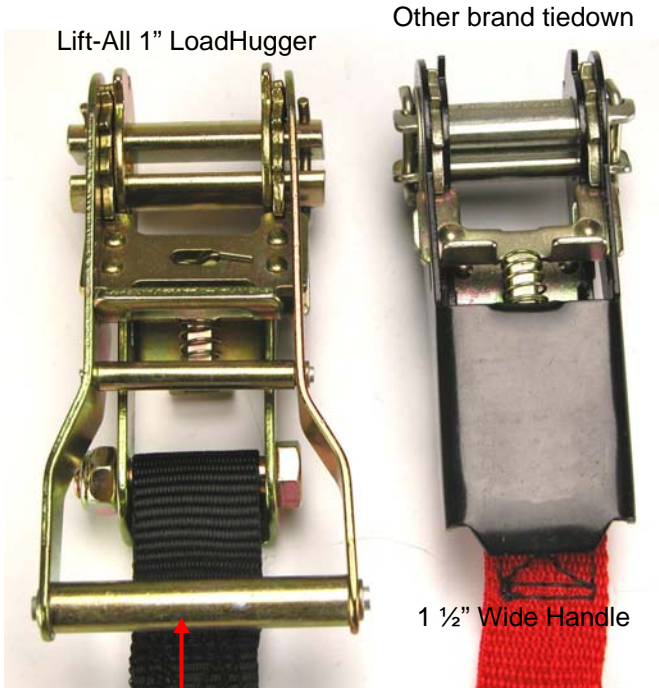
Lift-All uses long, wide (2 1/4") handle for better grip
