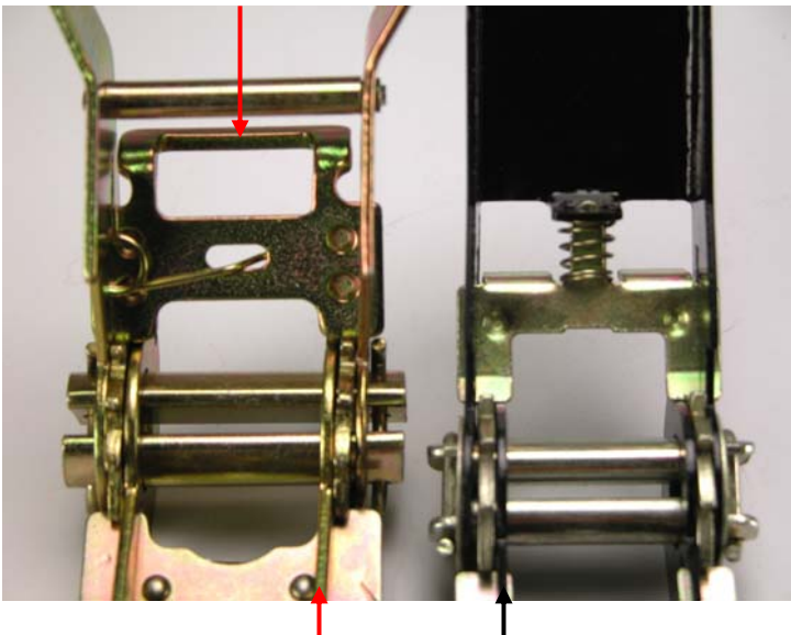
Thickness of steel used in ratchet body and handle
