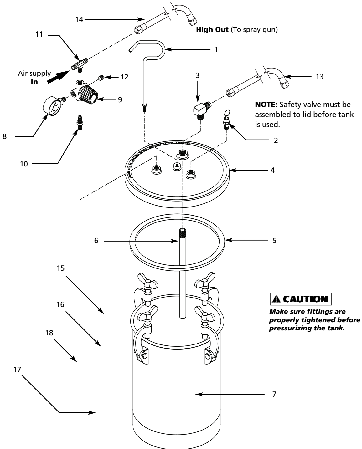
Figure 7 — Repair Parts Illustration
