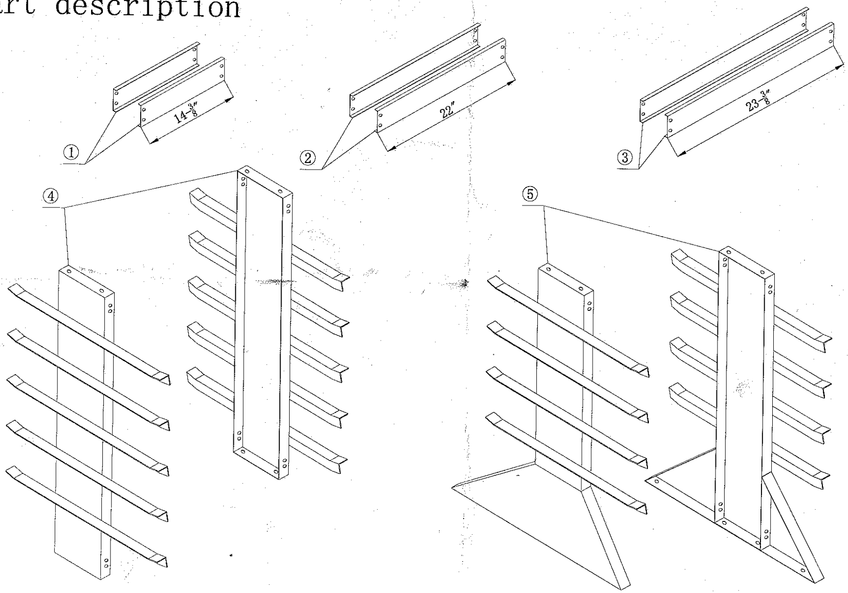
①: Small support bracket ②: Medium support bracket ③: Large support bracket ④: Upper body ⑤: lower
