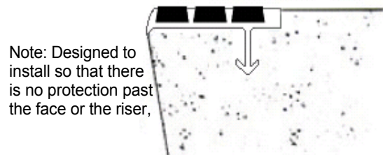
Detail - Sure hold anchor in concrete step
